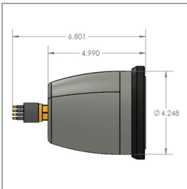
Dimensional drawing
